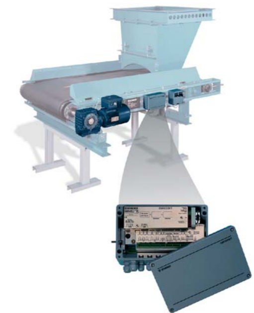
2 Dosierbandwaage in MechaTronik-Ausführung 2 Weighbelt feeder with MechaTronik System technology
